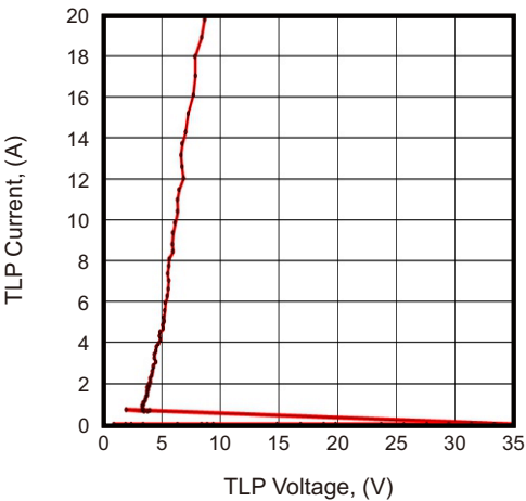
Fig.4 - TLP- Positive Pulse
